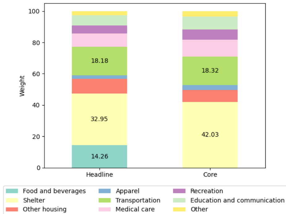
Figure 1: CPI Weights
