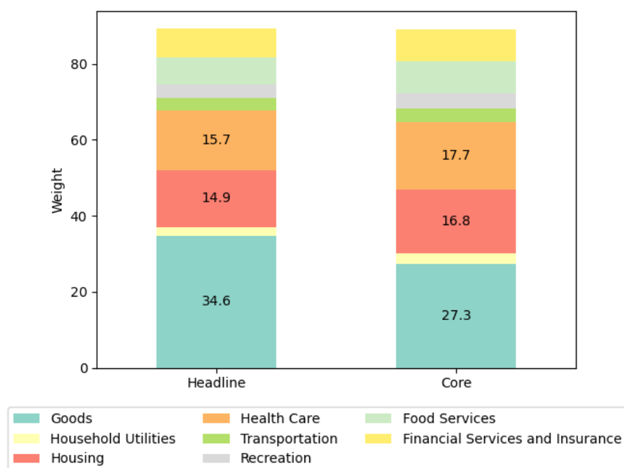
Figure 2: PCE Weights
